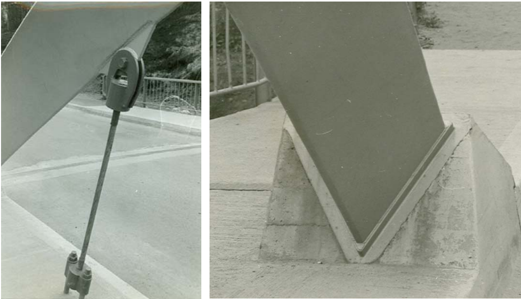
Fig. 8. Hanger and end of arch at Steinkjer.
