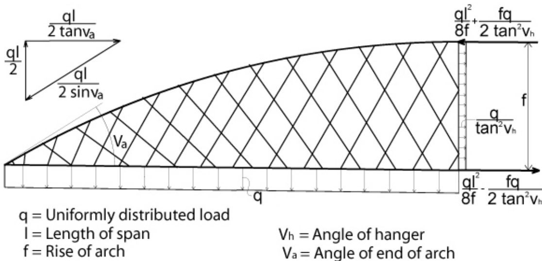
Fig. 11. Axial forces in network arches.
