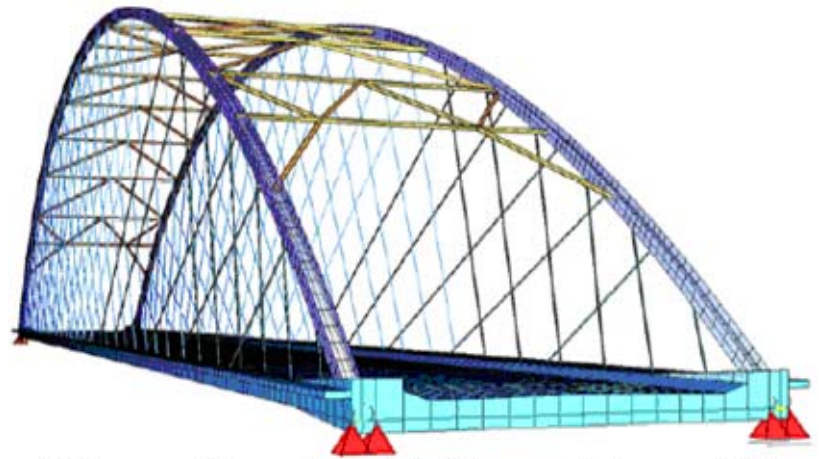
View of the 3-D FEM model used for calculations that can be found at http://fag.grm.hia.no/fagstoff/pert/
