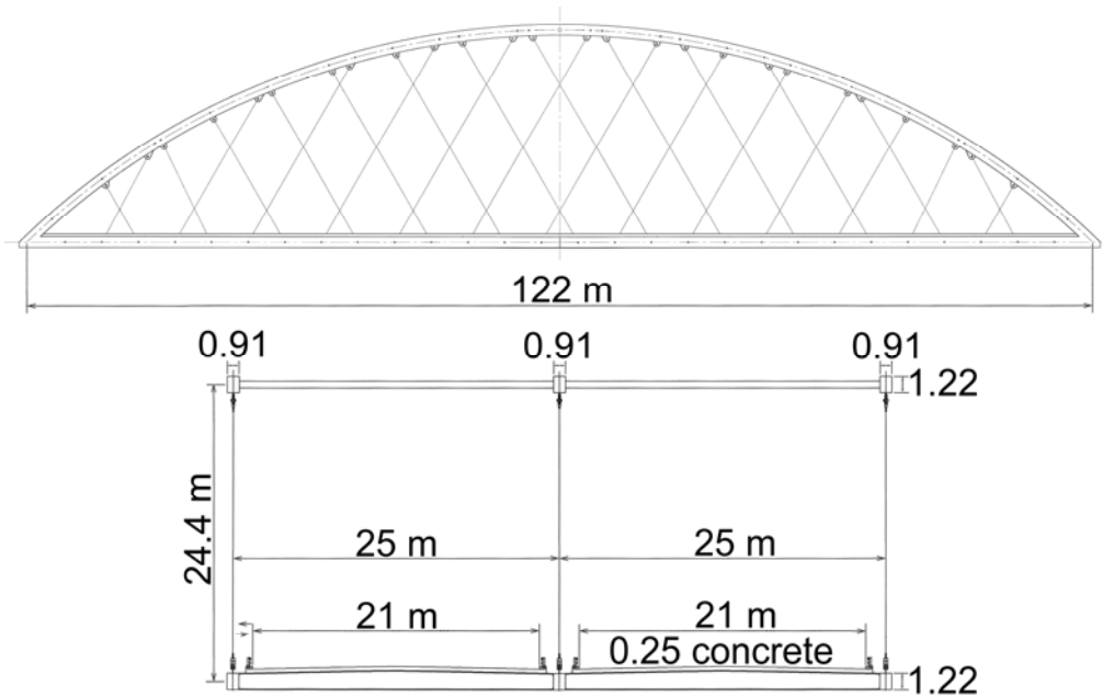
Fig. 49. A network arch in Providence, USA.
