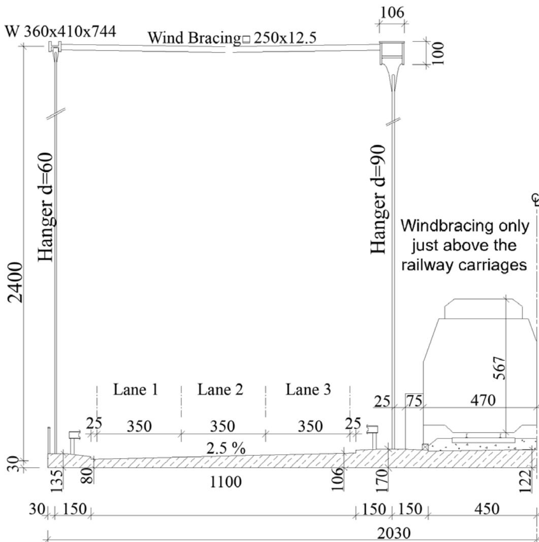
Fig. 42. Network arch bridge for road and rail.
