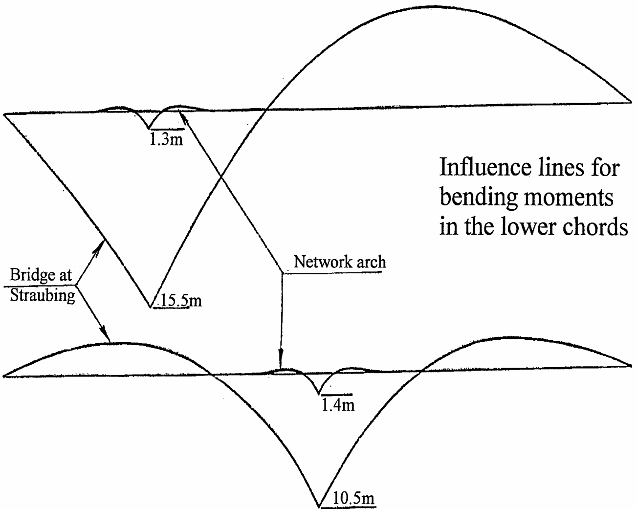
Fig. 14. Influence lines for the two arch bridges in fig. 13.
