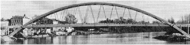
The longest Nielsen bridge. Castelmoron 1933. Span 145 m.
