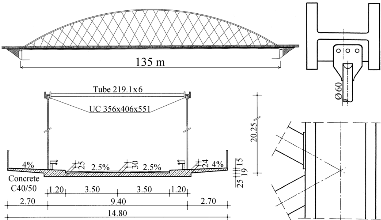
Fig. 18. A network arch between two Norwegian islands.
